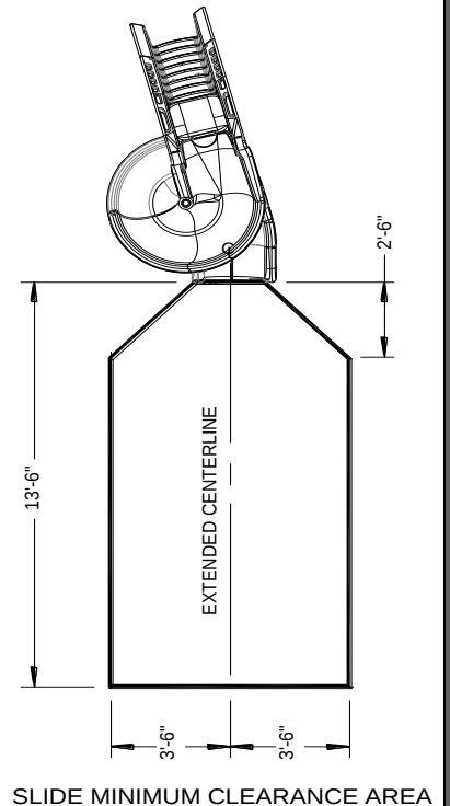
SLIDE MINIMUM CLEARANCE AREA
